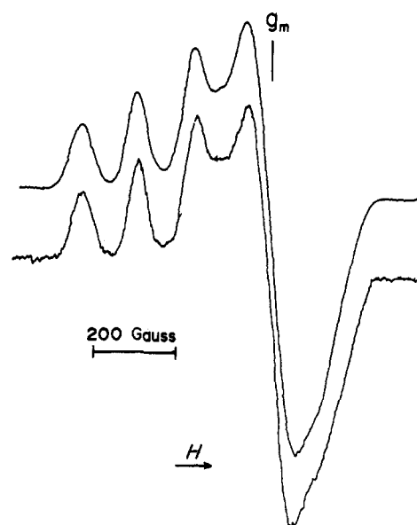
Figure 2. Electron paramagnetic resonance spectra of the superoxide dismutase from bovine erythrocytes (upper signal) is here compared with that of the enzyme isolated from bovine heart muscle (lower signal). The erythrocyte enzyme was at 47 mg/ml and the heart enzyme was at 8 mg/ml. Both were in 0.05 M potassium phosphate at pH 7.8. Other conditions for the erythrocyte and heart enzymes respectively were: microwave frequency, 9.082 and 9.101 GHz; microwave power, 10 and 25 mW; modulation amplitude, 4 and 3.2 G; scan rate, 500 and 125 G/min; time constant, 0.03 and 1.0 sec; receiver gain, 500 and 8000; and sample temperature, 77 K. The values of the spectral parameters are g_m = 2.080 ; g_{\parallel} = 2.265 ; A_{\parallel} = 0.014 \text{ cm}^{-1} .
